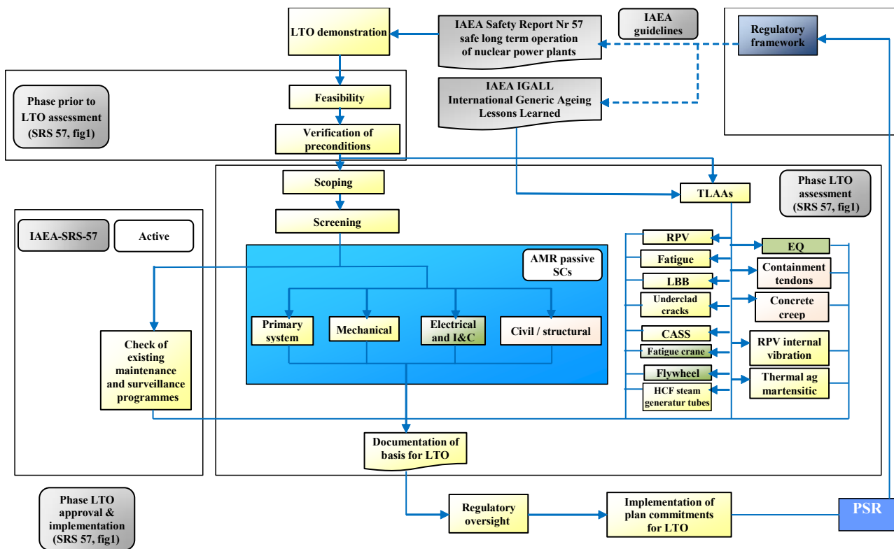
FIG. 12. Plan of approach for LTO projects (Swedish Radiation Safety Authority). AMR — ageing management review; CASS — cast austenitic stainless steel; EQ — equipment qualification; LBB — leak before break; SC — structure and component.
