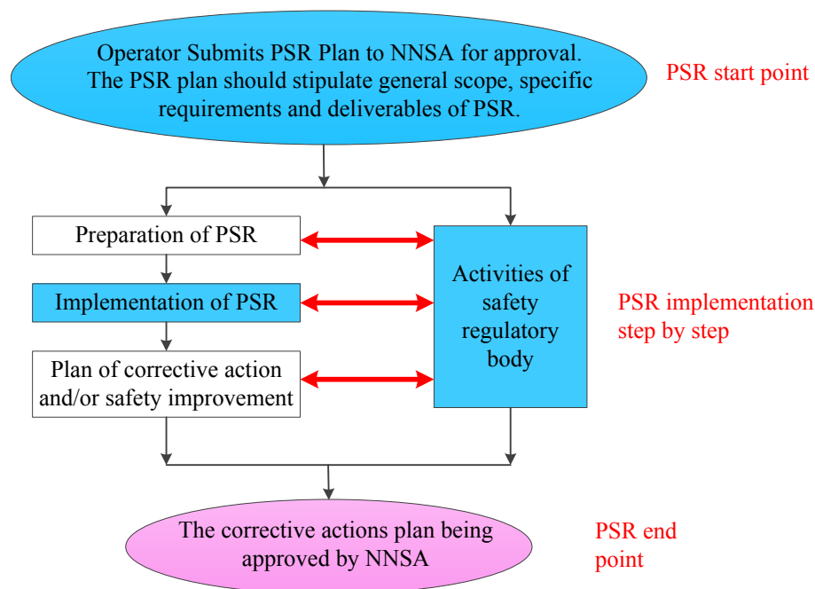
FIG. 63. Generic flow chart for PSRs in Chinese nuclear power plants. NNSA — National Nuclear Safety Administration.
