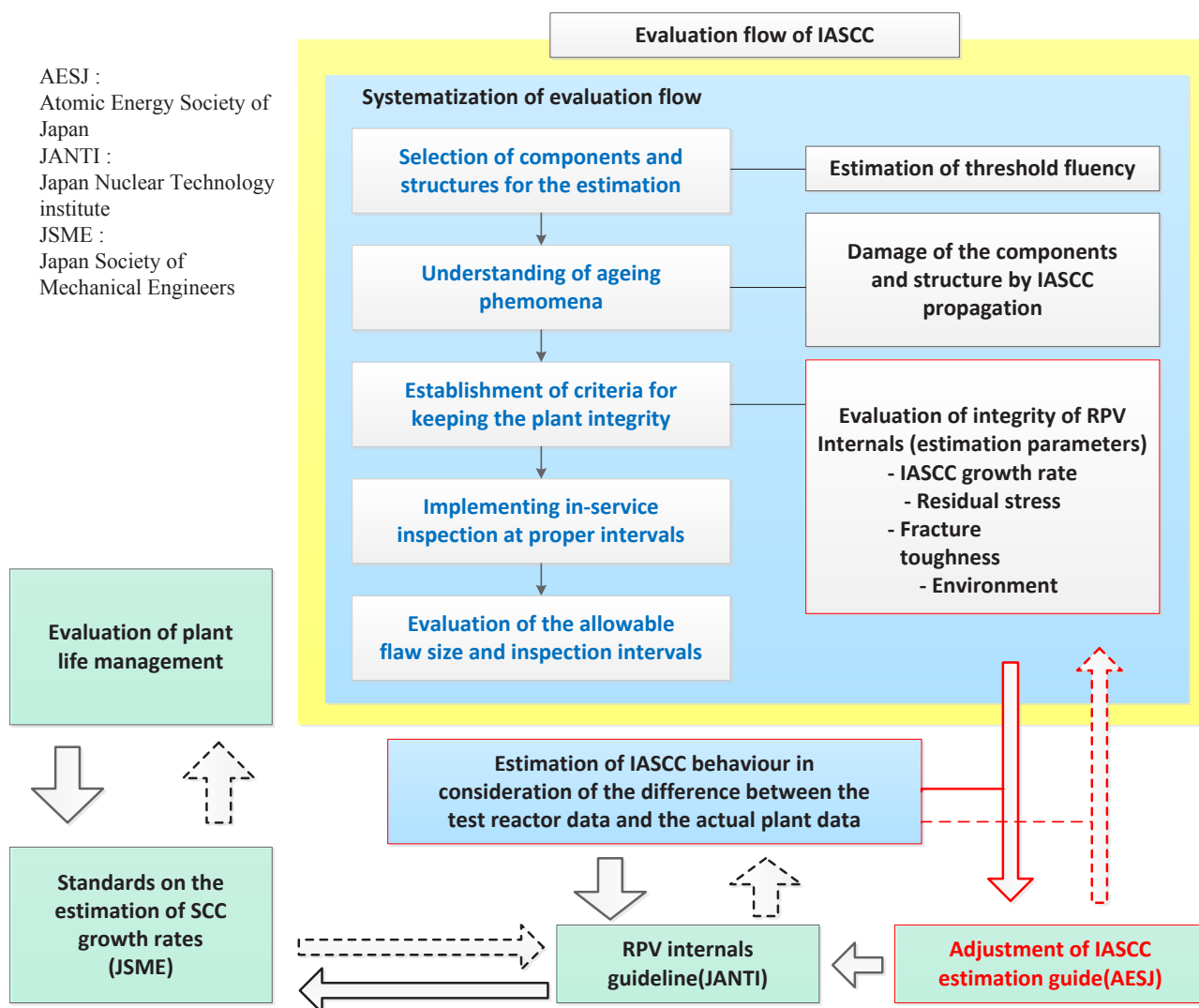
FIG. 22. IASCC evaluation scheme for RPV internals developed by the Tokyo Electric Power Company, Japan.
