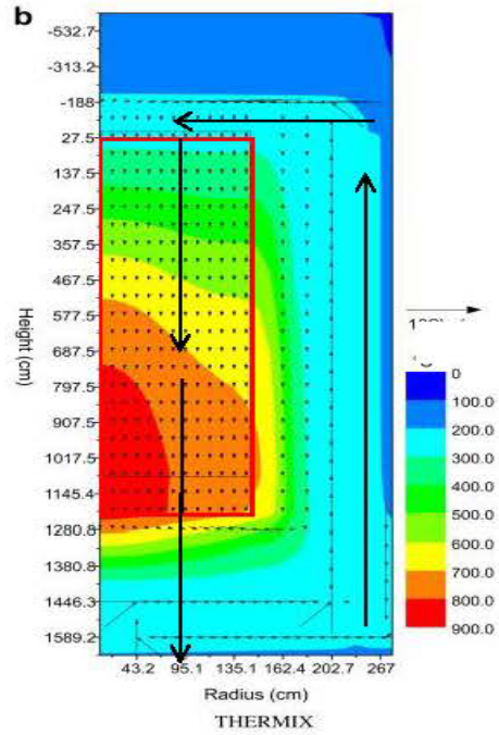
Figure 23. THERMIX graphite normal operation temperature profile (°C) of the HTR-PM 68 .
