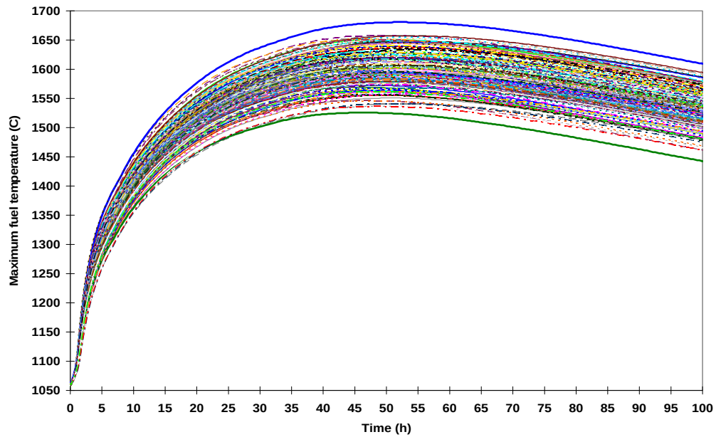
Figure 24. HTR-Module DLOFC maximum fuel temperature (°C) vs. time for 200 uncertainty variation cases 69 .
