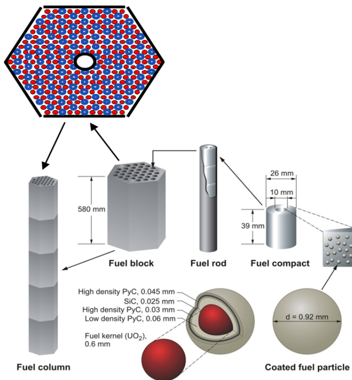
Figure 19. TRISO fuel, compact and block in a prismatic modular HTGR.
