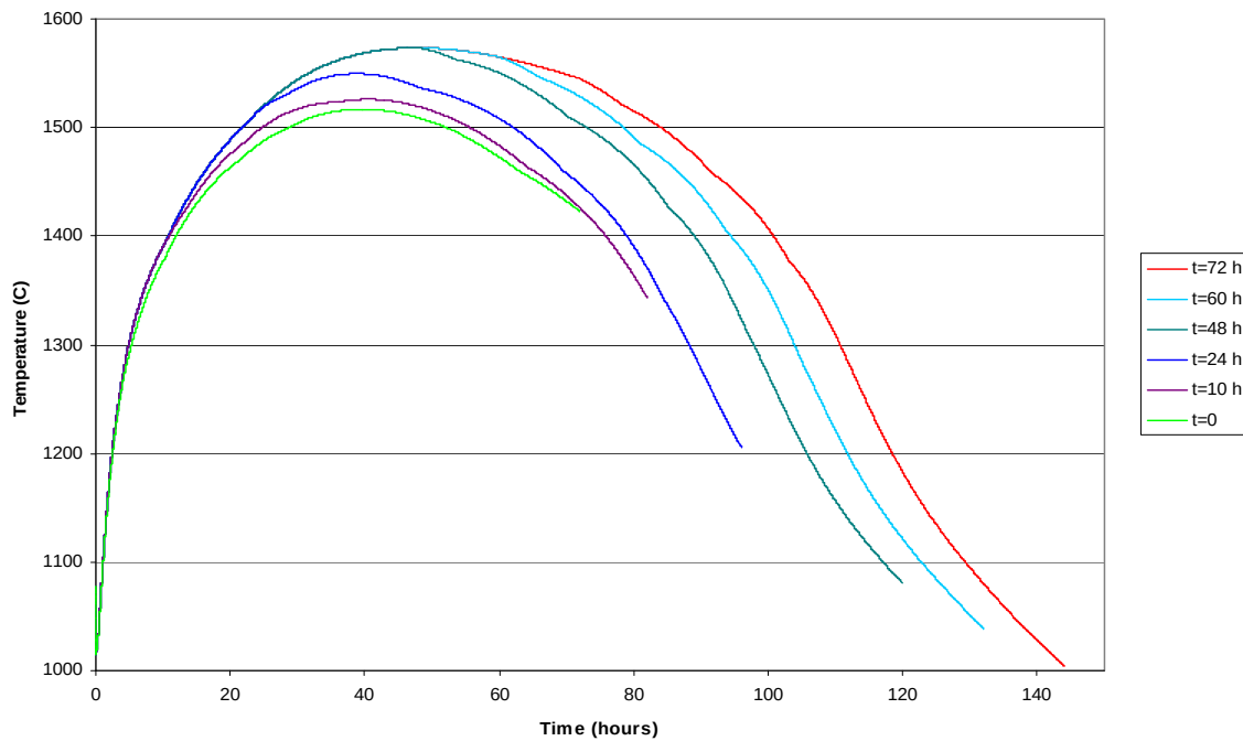
Figure 28. DLOFC maximum fuel temperature (°C) for the PBMR-400 for four air ingress start time variations 71 .
