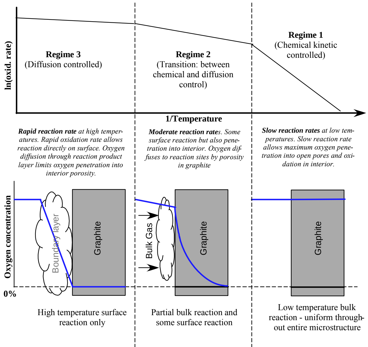
Figure 3. Three regime zones representing the variation in oxidation rate with temperature in bulk graphite 4,5,11 . Regimes are dependent upon flow conditions, temperature, and individual graphite microstructure.
