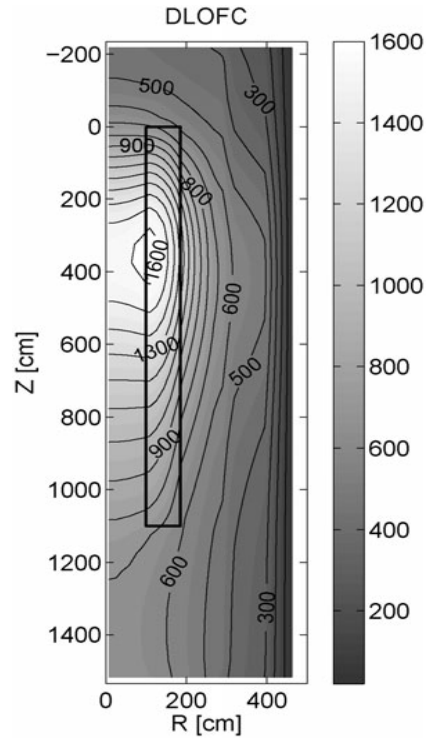
Figure 26. DALTON-THERMIX graphite temperature profile (°C) of the PBMR-400 at 100 h 70 .
