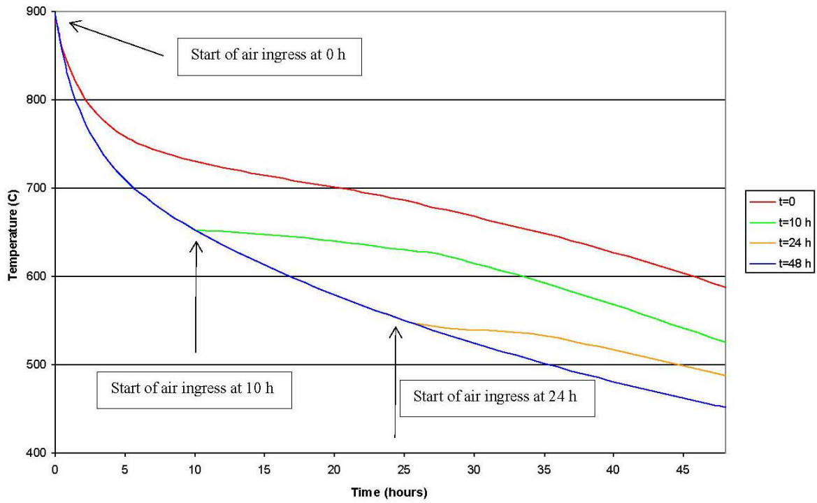
Figure 27. DLOFC bottom graphite temperature (°C) for the PBMR-400 for four air ingress start time variations 71 .
