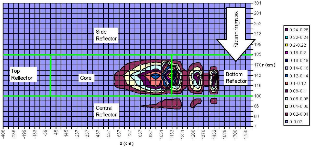
Figure 30. Spatial distribution of graphite oxidized (kg) in the PBMR-400 at 72 h: steam ingress at bottom break location at 0.277 kg/s 71 .
