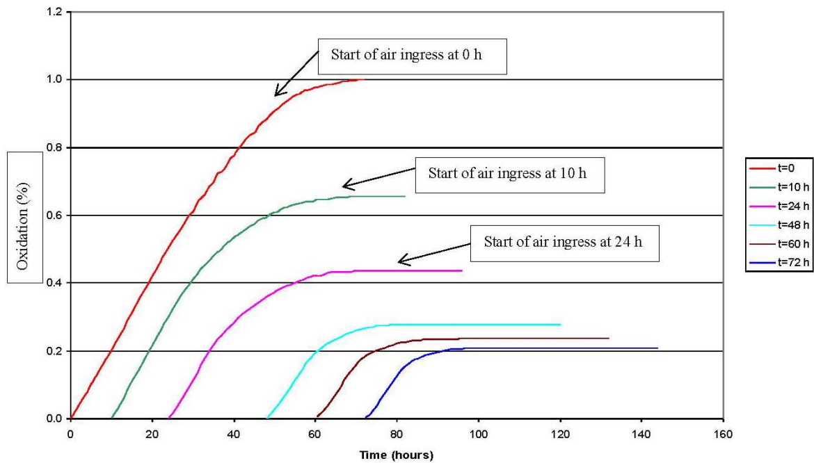
Figure 32. Graphite oxidation (%) in the bottom reflector vs. time for 6 air ingress start time variations 71 .
