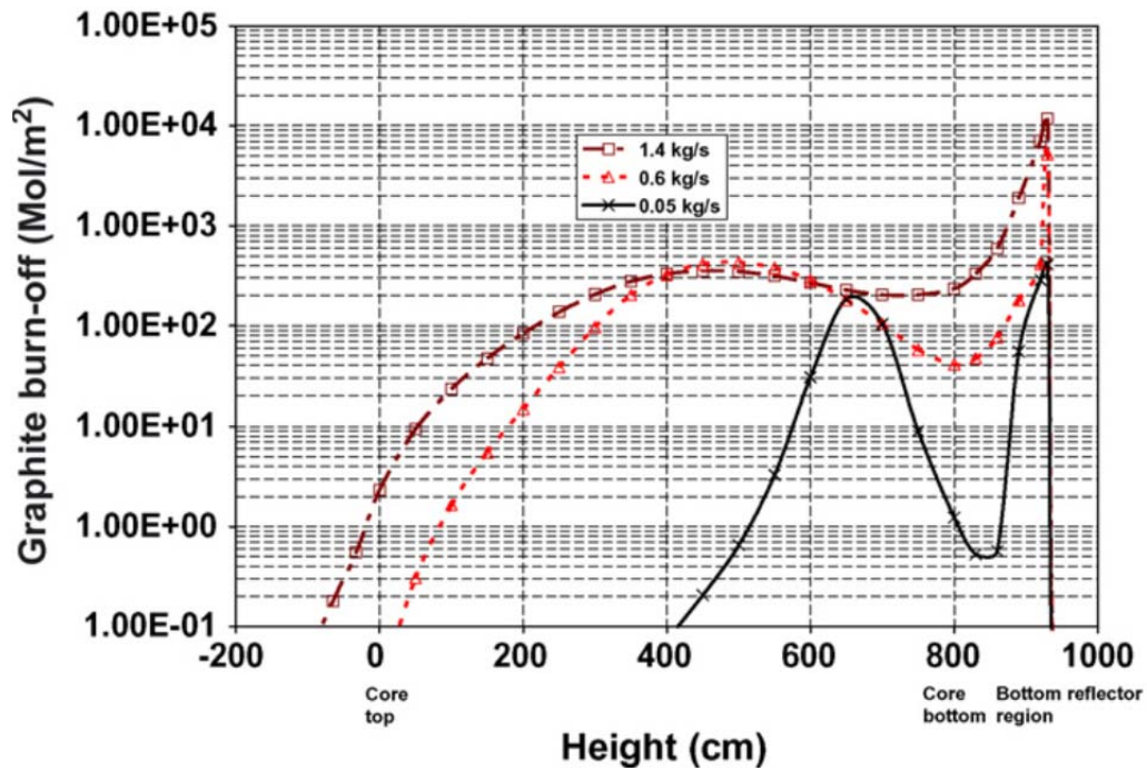
Figure 35. Axial graphite oxidation distribution ( \text{Mol/m}^2 ) in the ANTARES reactor at 70 h for various air flow rates 73 . ( 1000 \text{ Mol/m}^2 = 1.2 \text{ g/cm}^2 )
