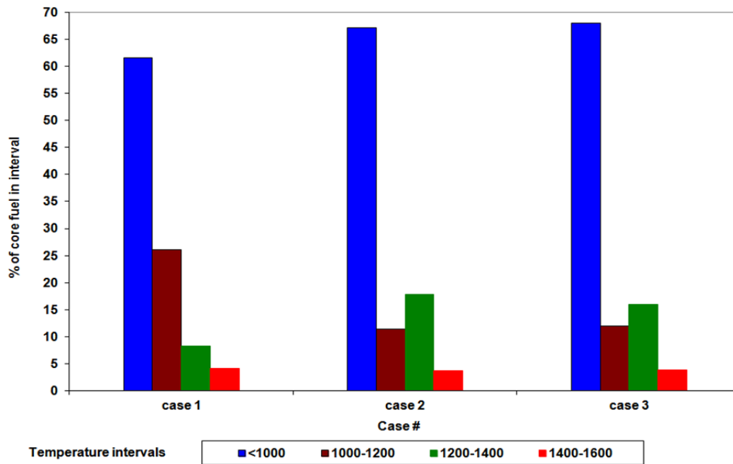
Figure 25. Maximum graphite temperature volumetric distribution for three HTR-Module DLOFC cases at the time of peak fuel temperatures (% of total fuel volume) 67 .
