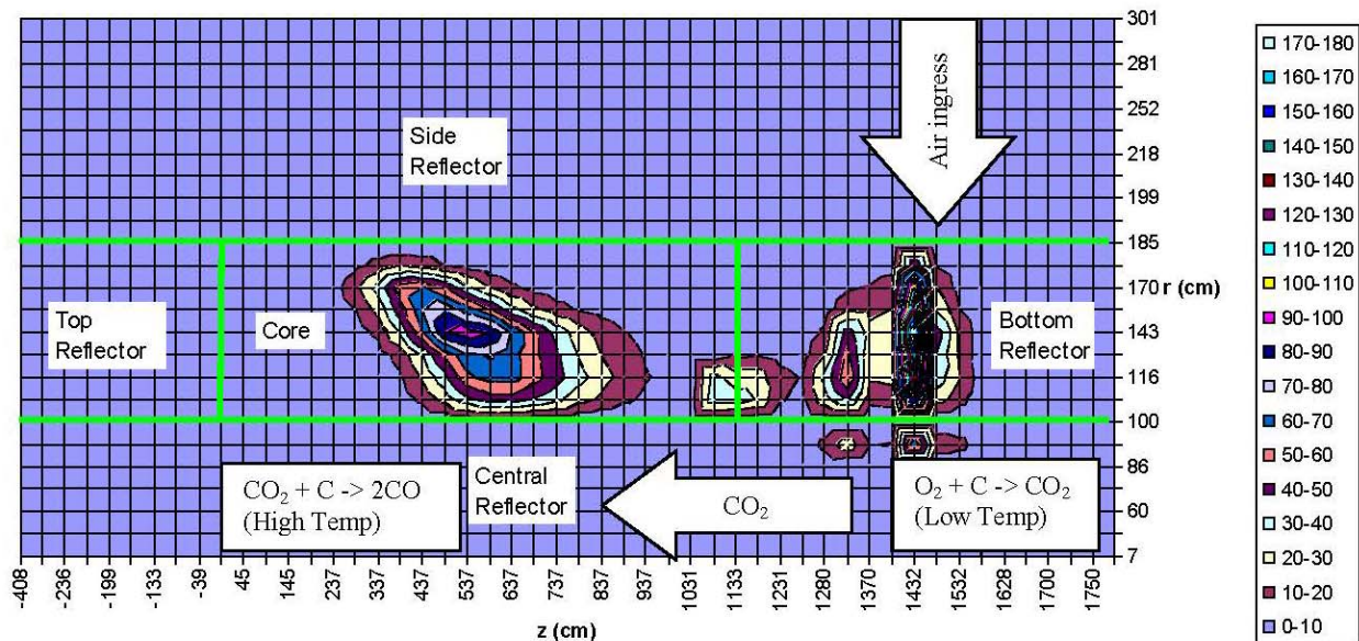
Figure 29. Spatial distribution of graphite oxidized (kg) in the PBMR-400 at 72 h: air ingress at bottom break location at 0.208 kg/s 71 .
