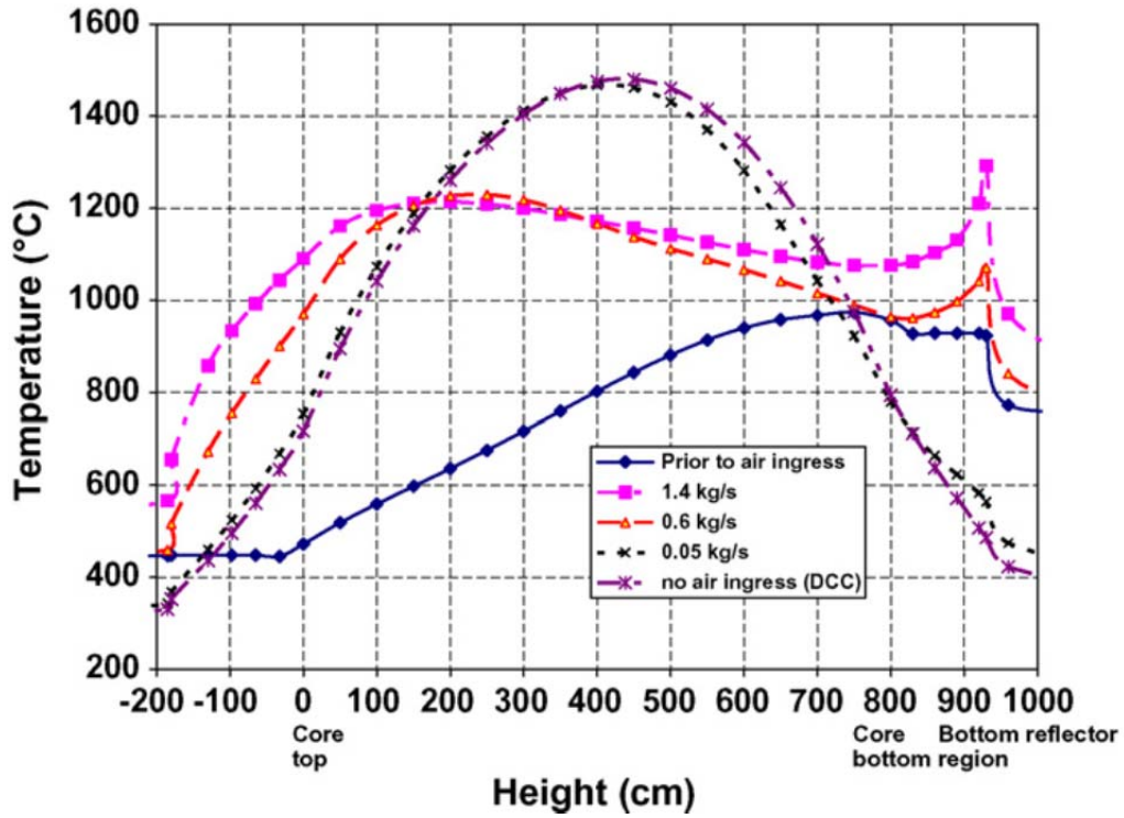
Figure 34. Axial temperature ( ^{\circ}\text{C} ) distribution in the ANTARES reactor at 70 h for various air flow rates 73 .
