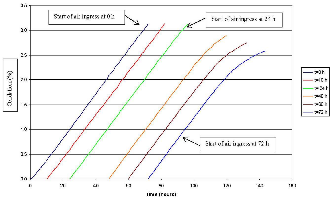
Figure 33. Graphite oxidation (%) in the active core region vs. time for 6 air ingress start time variations 71 .
