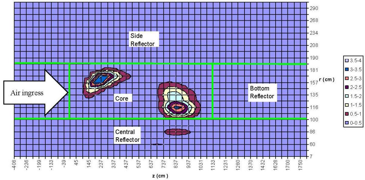
Figure 31. Spatial distribution of graphite oxidized (kg) in the PBMR-400 at 72 h: air ingress at top break location at 0.009 \text{ kg/s}^{71} .
