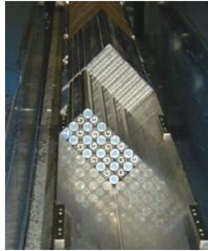
FIG. 3. Example of a loading pattern
