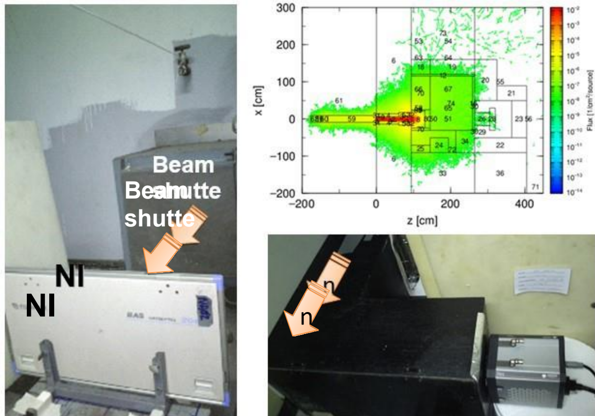
Fig. 3 Beam facility: Photos of the beam facility and simulation of neutron flux
