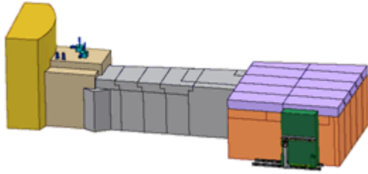
Thermal Neutron Imaging Facility at CARR (Under Construction)
