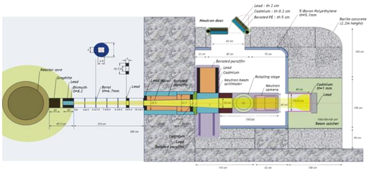
Fig.2 Proposed upgrade NR station at TRR-1/M1 indicated wider working space, more effective shutter, three collimators behind reactor wall and safety
