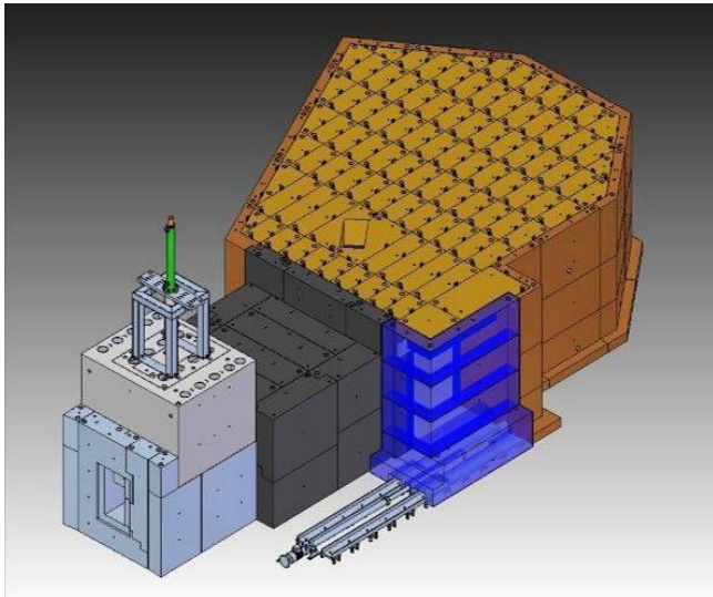
NEW NRAD FACILITY (SIMULATION) TO BE IN OPERATION FROM FEB 2014
