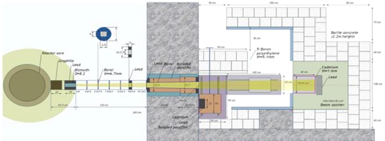
Fig.1 Current NR station at TRR-1/M1 indicated limit working space, small shutter and no behind reactor wall collimator
