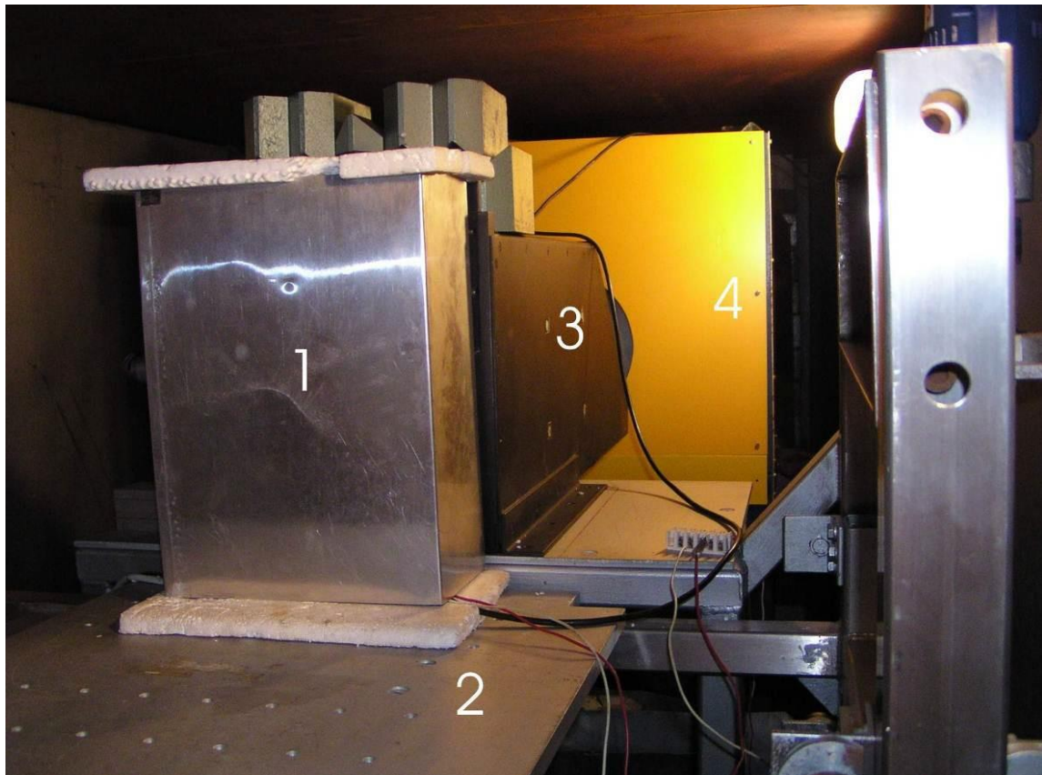
The inside view of the NGRS neutron and gamma radiography station. The thermal chamber (1) on the object table (2), the optical system box (3) and the beam trap (4) are visible.
