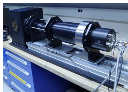
Figure 11. Large CCD, 10 kPixel x 10 kPixel, FOV 10 cm x 10 cm, Scintillator 20 \mu\text{m} Gadax. Overall resolution 20 \mu\text{m} .
