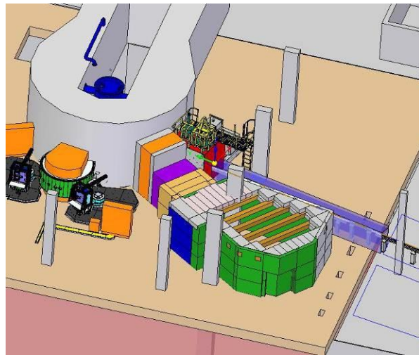
NEW NRAD FACILITY (SIMULATION) TO BE IN OPERATION FROM FEB 2014
