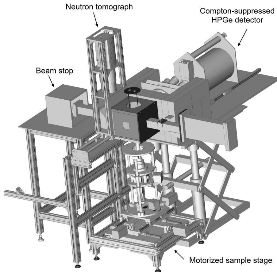
Irradiation facility (model)
