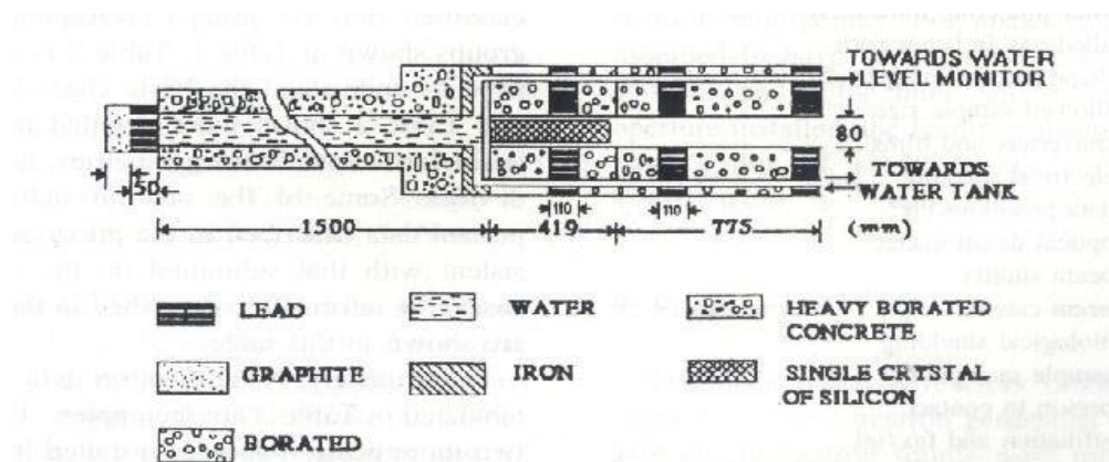
Fig. 1. Sectional view of neutron beam facility in the tangential beam port at Dalat Research Reactor.
