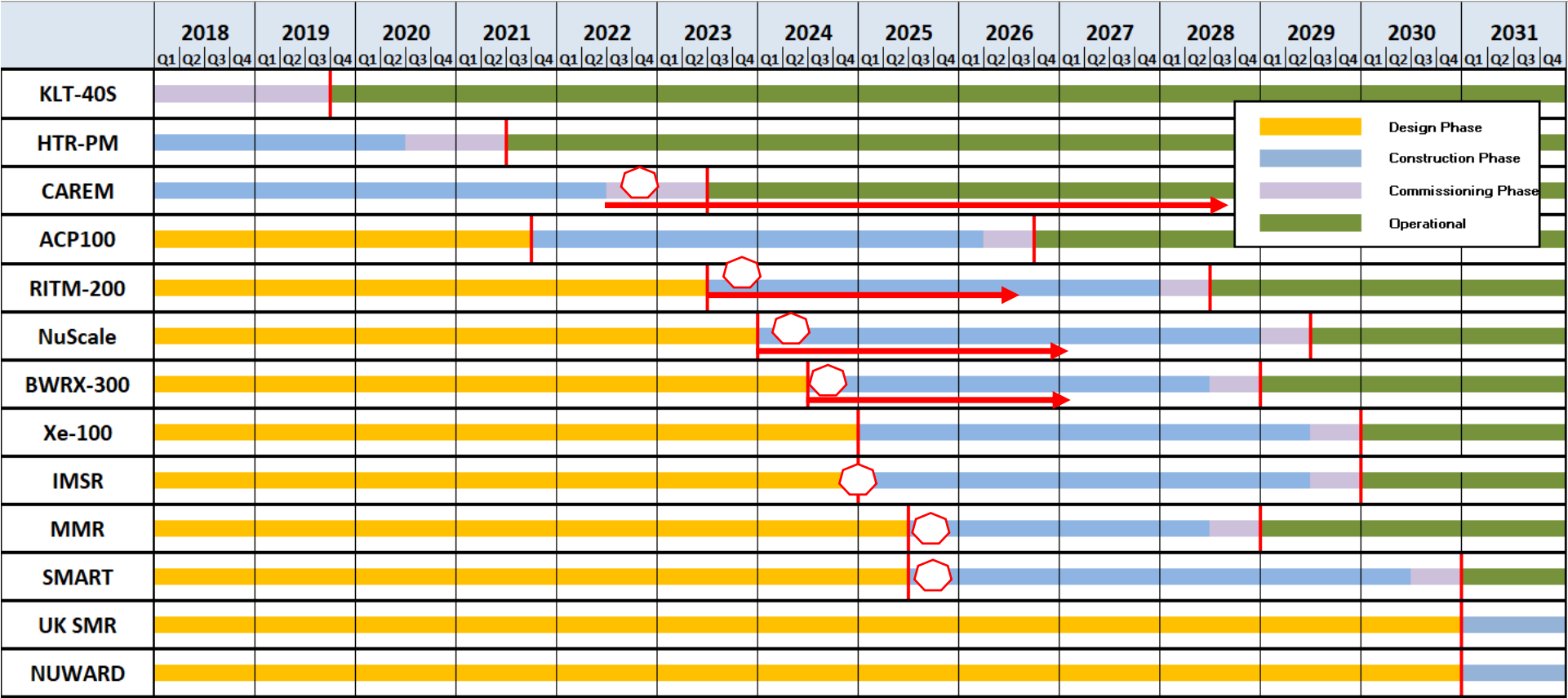
Initial Timeline of Deployment (2021) of some SMR designs up to 2030/2031
